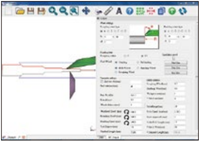
Roughing Wheel at 10°
